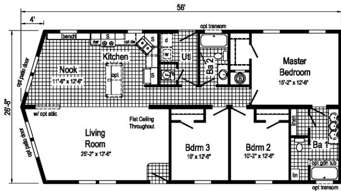
RG751-A 2856 Approx. 1440 Sq. Ft.
