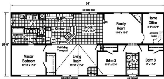
RG763-A 2864 Approx. 1707 Sq. Ft.
